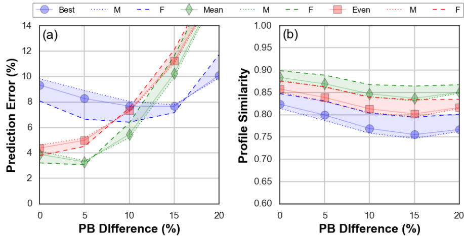
Fig. 4. Prediction error (a) and pacing profile similarity (b) vs. PB Difference for Best , Mean , and Even strategies, and for all runners and men and women.
