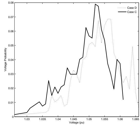
Fig. 9. The voltage PDF of the rurally located bus in WR 4 plotted for the two control cases. Voltages shift toward higher values as more terminal voltage control is enabled.
